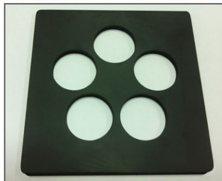
32mm Flange Holder for Sub-Ducts in Manhole
